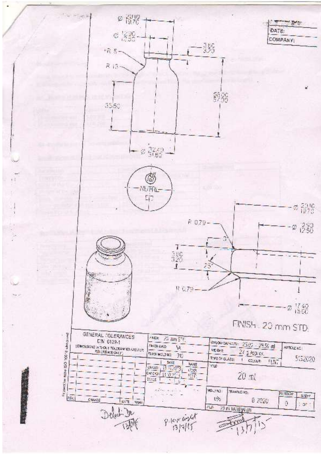
Drawing-II for 20ml Vials.
